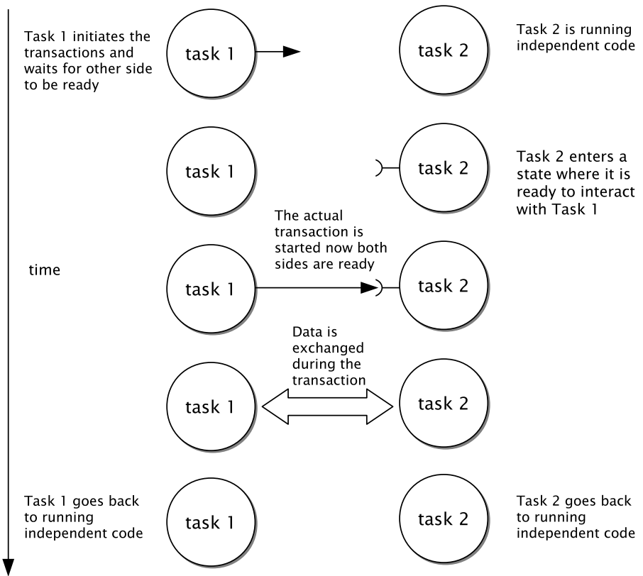
Figure 2: Two tasks performing a transaction
