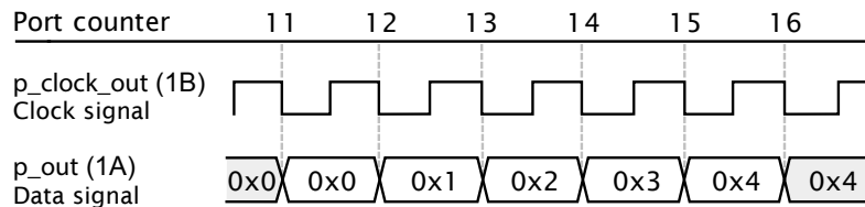
Figure 22: Waveform diagram
