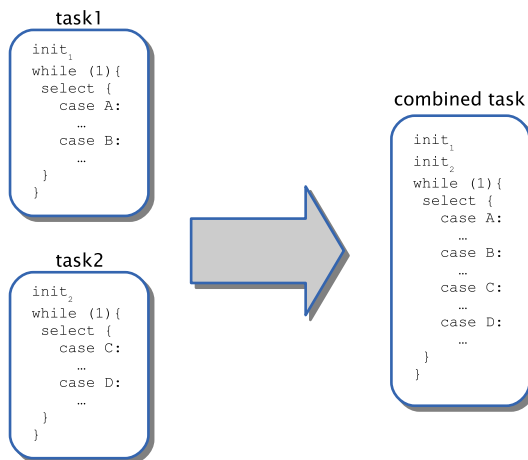
Figure 11: Combining several tasks
