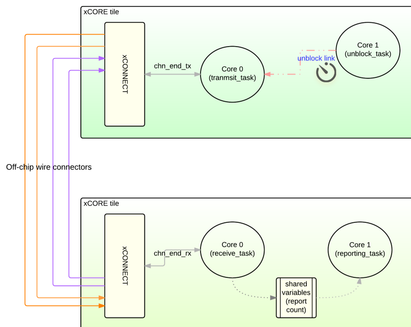
Figure 2: Demo application tasks
