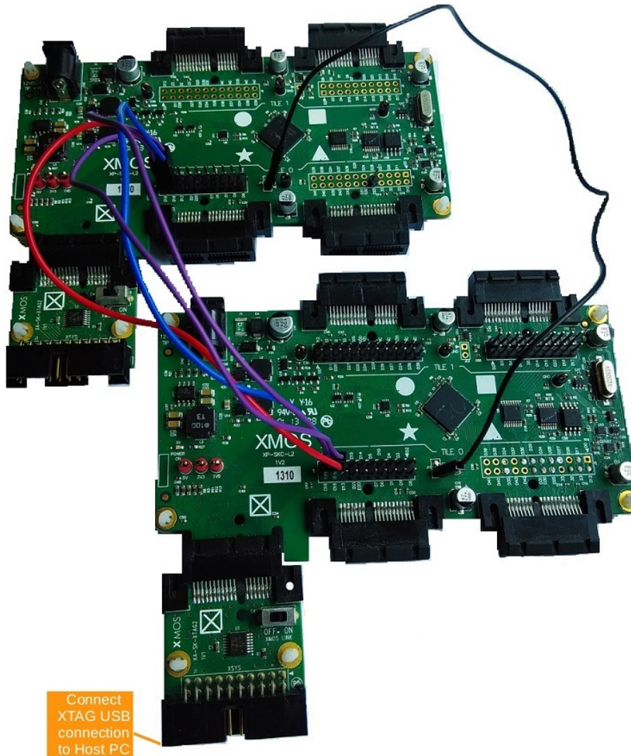
Figure 3: 2-wire XMOS xCORE-L16 sliceKIT set up for off-chip xCONNECT communication
