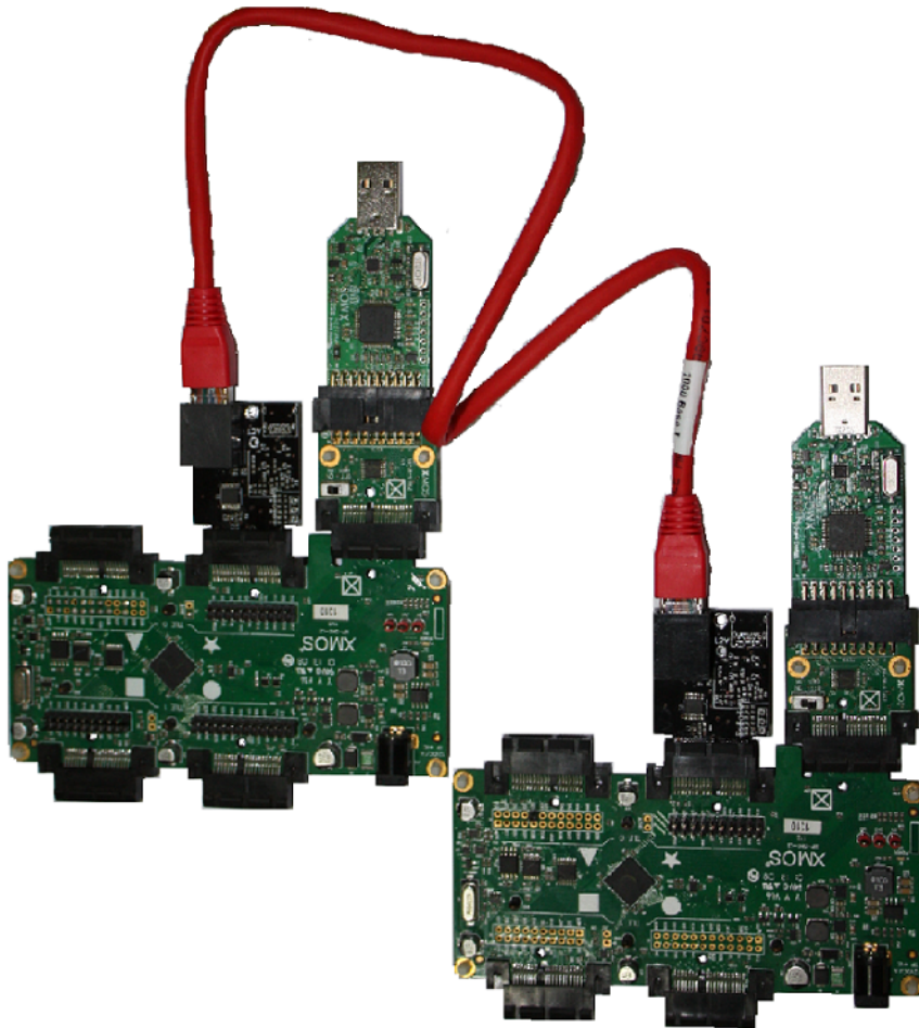
Figure 4: Two-wire xCONNECT communication set up using RJ45-type LVDS sliceCARD connected to xCORE-L16 sliceKITS
