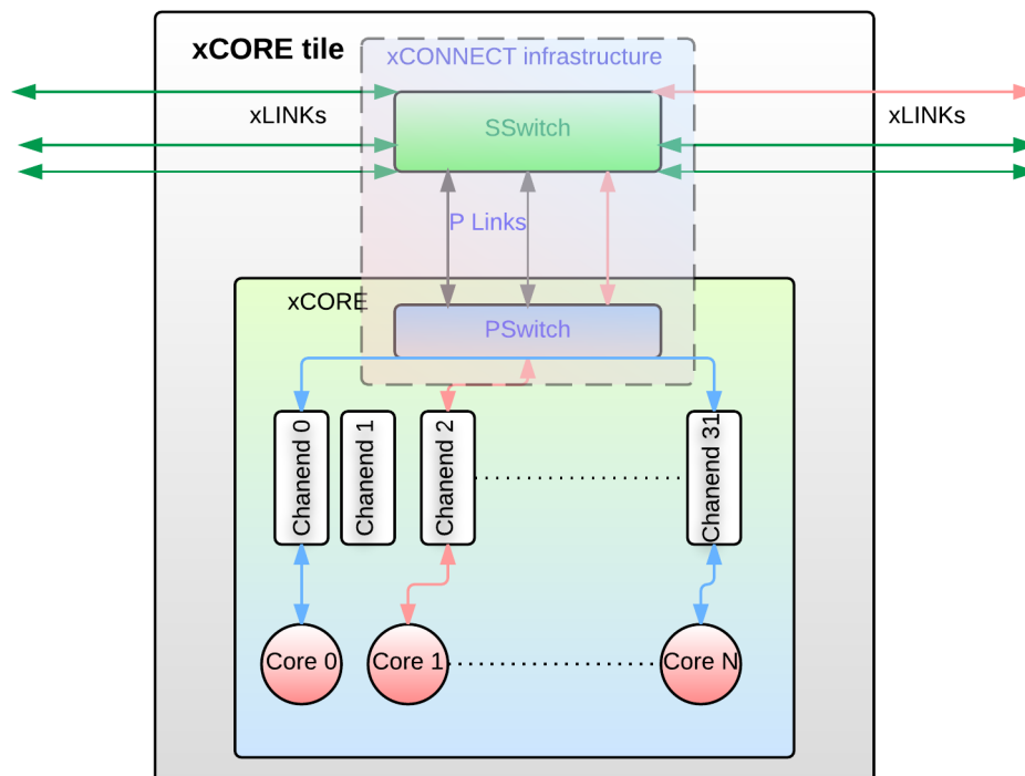
Figure 1: Block diagram of an xCORE tile
