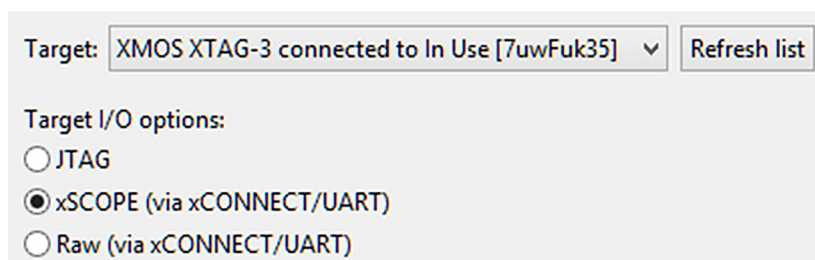
Figure 6: xTIMEcomposer xSCOPE configuration
